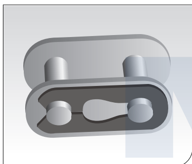
Connecting link with half-close spring clip
